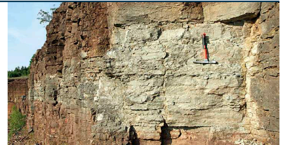
The interval with the grey, 1.5-meter-thick 'Täljsten' reflects a prominent sea level drop and is enriched in extraterrestrial chromite grains. (Photo: Anders Lindskog).
