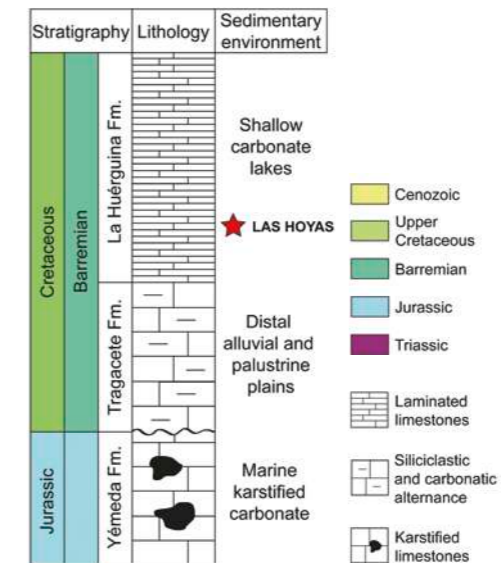
Paleogeographic, geological and sedimentary setting of Las Hoyas in the Iberian Plate, remarking its location (red star) within the Barremian deposits.
