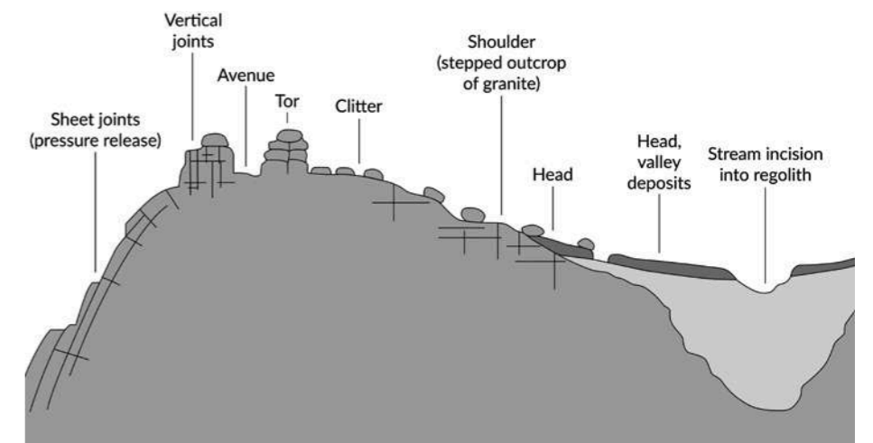
Diversity of granite landforms and surface deposits in relation to jointing and topography, after Gunnell and Jarman (2020).
