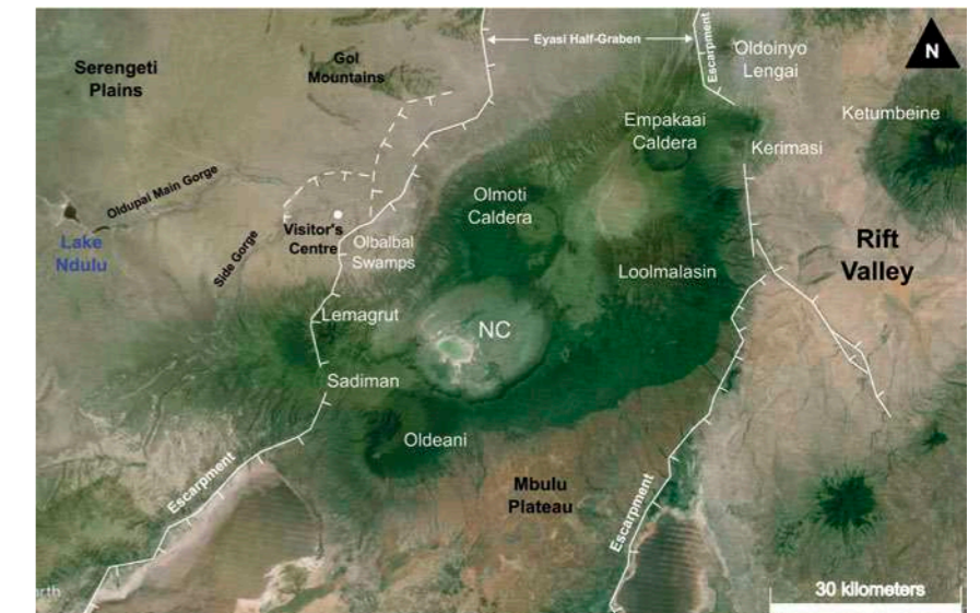
Geological setting of the Ngorongoro Crater (NC), Ngorongoro Volcanic Highlands, and the branches of Gregory Rift (modified from Scoon, 2018). Source: Landsat/Copernicus. Google Earth.
