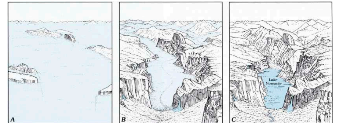
Evolution of the Yosemite Valley from the times of major glaciation to the early Holocene (after Huber, 1989).
