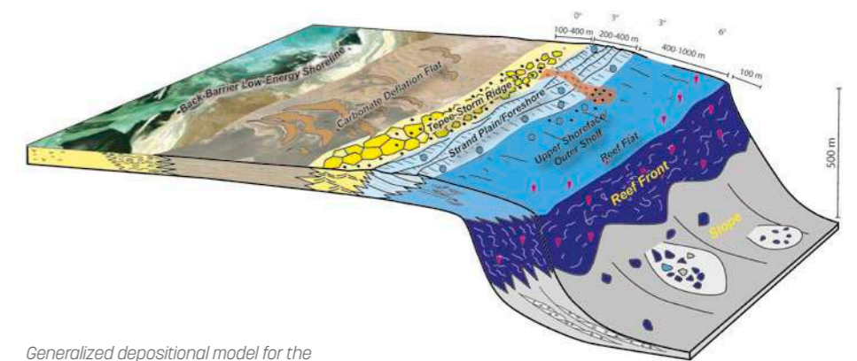
Generalized depositional model for the Capitan Reef and associated shelf and slope-basin deposits.
