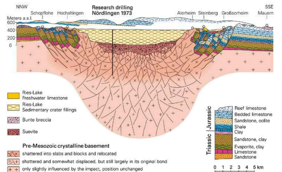
Geological Cross section of the Ries crater with reconstructed pre-impact landscape (Bavarian Environment Agency (LfU)).
