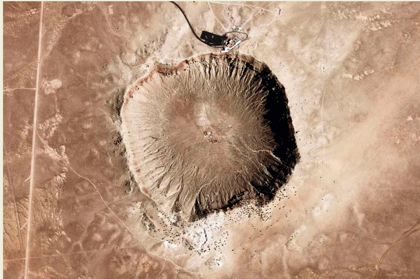
Satellite image of Meteor Crater. Credit: NASA Earth Observatory.
