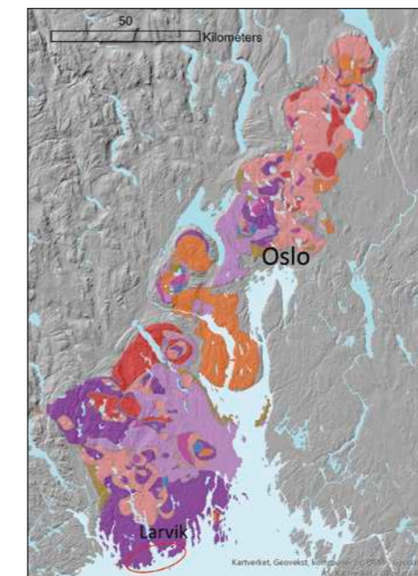
Map of the Carboniferous - Permian Oslo Igneous Province.
