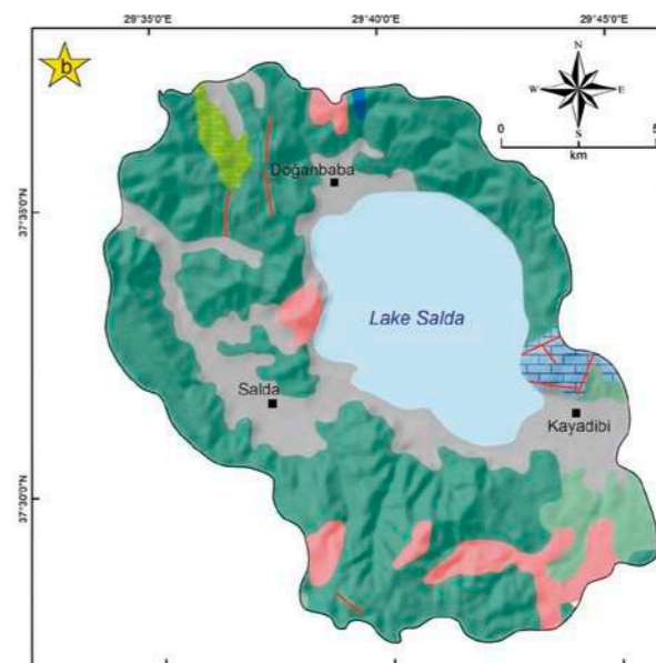
Location map (a) and rocks in the drainage area of Lake Salda (b) following the geological map at scale of 1/500 000 published in 2002 by Turkish Geological Survey (MTA).
