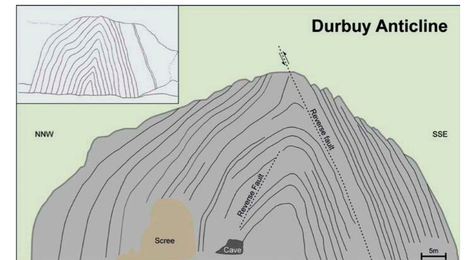
The original sketch of the Durbuy Anticline from the publication by d'Omalius d'Halloy (upper left-hand corner) in comparison with a modern representation.
