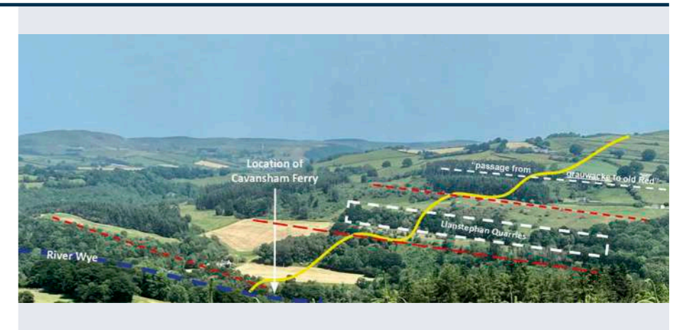
"Low-terrace shaped ridges of grey rock", Cavansham Ferry to Trewerne Hills. Yellow marks the line of Murchison's section, red dashed lines are ridge crests.
