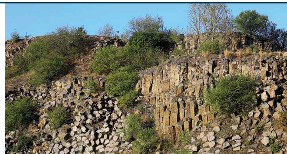
Columnar jointed basalt of the former lava lake within the Zalahaláp maar-diatreme craters demonstrates complex cooling history of lava. Photo by: Barnabás Korbély.
