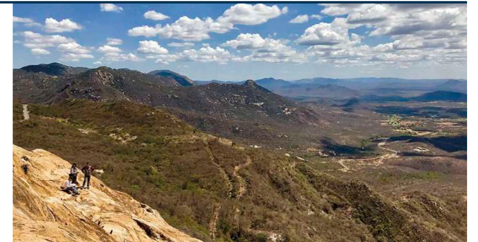
Looking east along the southern margin of the Patos SZ, where deformed Ediacaran granitic plutons form hills in the semi-arid landscape of NE Brazil.
