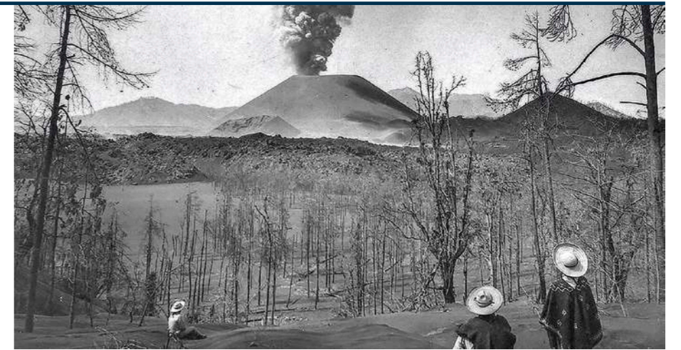
Local indigenous residents observe Parícutin volcano, in march 1944. Photo by Amo Brehme (U.S. National Archives, published in Foshag and González Reyna, 1956).
