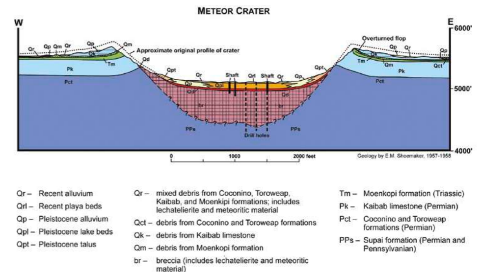
Geological cross-section of Meteor Crater. Credit: Kring (2017).
