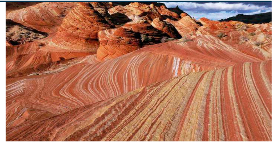
Vivid coloration follows aeolian laminae and strata leading towards The Wave at the Coyote Buttes. Image: V. Thompson.
