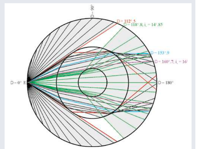
Visualisation of Lehmann's simplified earth model: The outer core focuses seismic waves creating a shadow zone, whereas the inner core acts as a diverging lens, shedding seismic energy into the shadow zone (Kölbl-Ebert, 2001).
