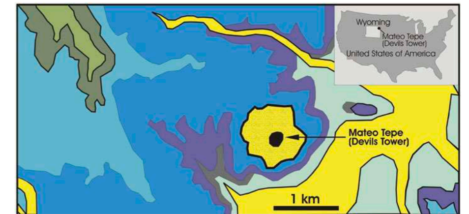
Devil's Tower Regional Geology, and Location
